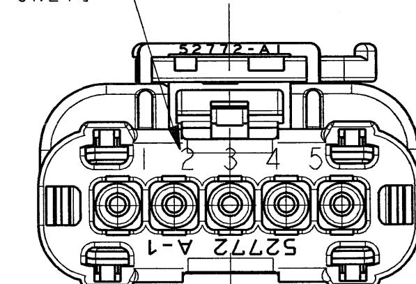
SEALED ASSEMBLY VIEWS SEE P/N CHART SHOWN WITH CPA
