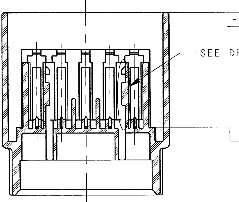
SECTION E-E FOR REFERENCE ONLY INSULATOR VIEWS
