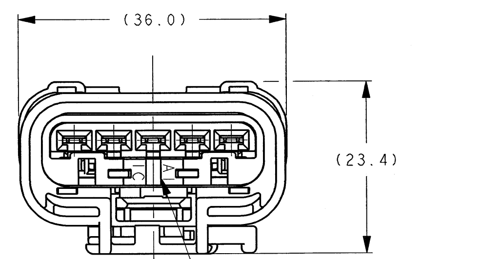
END VIEW W/CPA
