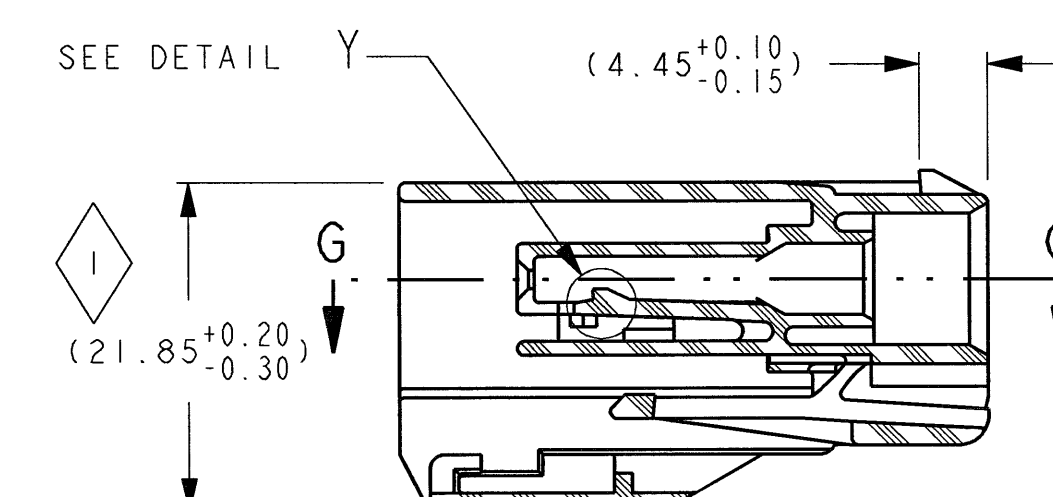
SECTION F-F
